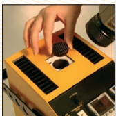
Black Body
